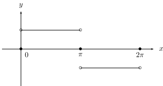
Figura 3.39: y = \operatorname{signo}(\operatorname{sen} x)
