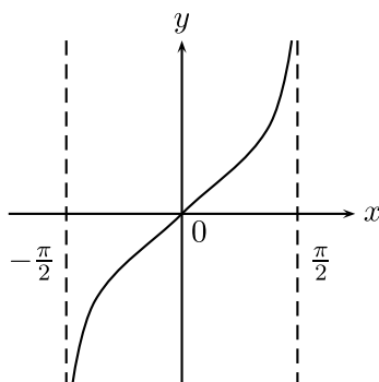
Figura 3.33: y = \tan x
